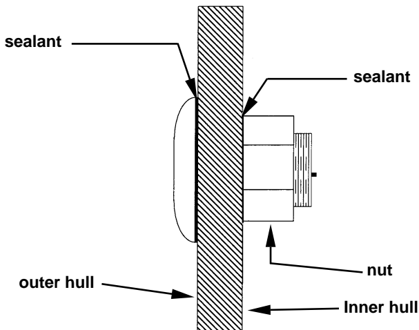
Cross section of transom showing EP-35 TH installed.
